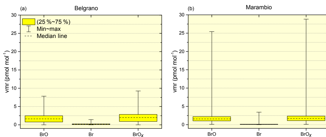
Figure 13. Statistical analysis of the reactive bromine and its partitioning estimated at Belgrano (a) and at Marambio (b) during the sunlit period of 2015. The vertical scale, which is the same in both plots, indicates the range of mixing ratios of BrO, Br and \text{BrO}_x at both stations ( \text{SZA} < 75^\circ ). The legend applies to both figures, where the whiskers display the range of the maximum and minimum vmr, the boxes in dark yellow provide the vmr ranges of 25–75 % of the data and dashed lines depict the median vmr.
