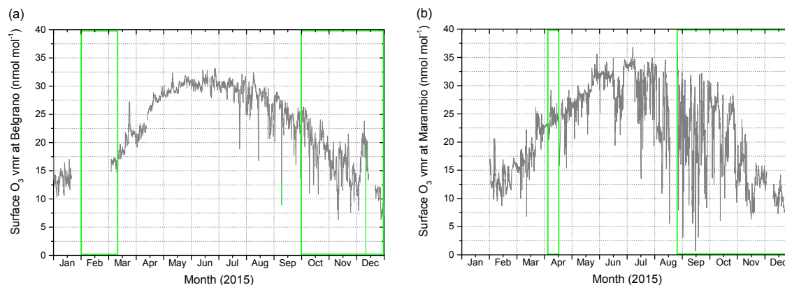
Figure 6. The 2015 near-surface ozone observations at the Belgrano (a) and Marambio (b) research stations. Note the same vertical scale in both plots. Both data sets were gathered by in situ O_3 observations made by INTA (at Belgrano) and by the Argentinian Meteorological Service (at Marambio). The periods with MAX-DOAS data ( SZA < 75^\circ ) at each station are contained within the green boxes.
