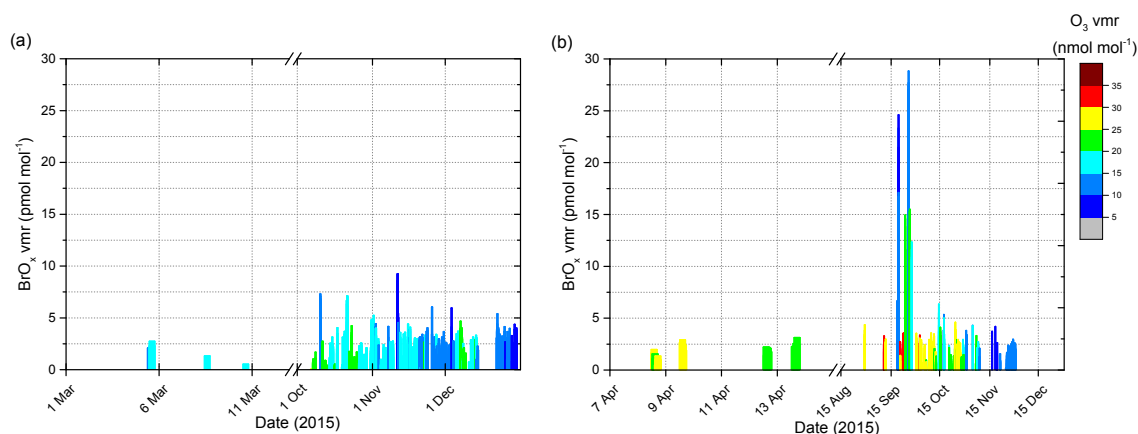
Figure 12. Reactive bromine in the low troposphere of Belgrano (a) and Marambio (b) under different \text{O}_3 regimes. The vertical scale depicts the \text{BrO}_x ( \text{Br} + \text{BrO} ) at each station and the color code refers to the collocated observed \text{O}_3 vmr. Note that the vertical scale and the color code apply to both figures. Only observations performed under low wind conditions ( < 6 \text{ m s}^{-1} ) and a \text{SZA} < 75^\circ are included.
